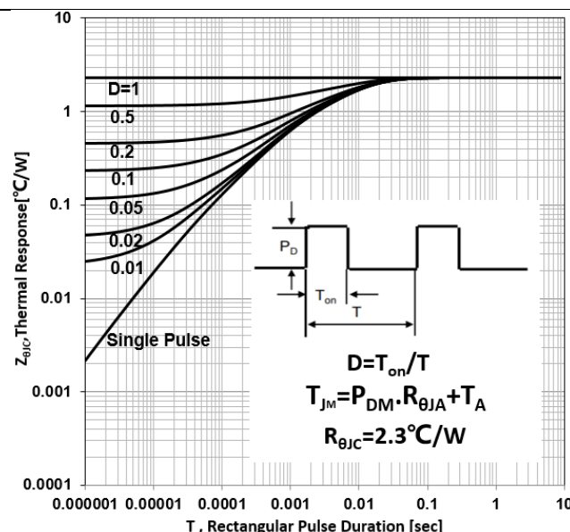
Figure 3b Max Thermal Impedance (TO-220F)
